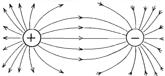
As the charges are moved apart, the connecting field-lines move apart and spread out unconstrained.
